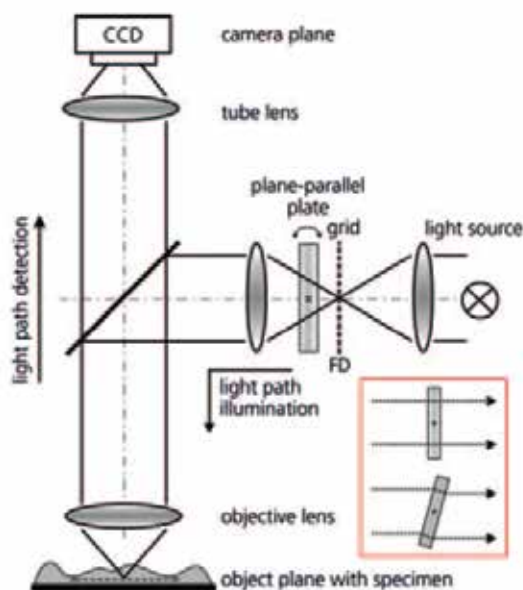
Figure 3: Beam path for structured illumination in a conventional fluorescence microscope (FD = field diaphragm plane). The inset shows the parallel movement of the projected grid resulting from tilting a plane-parallel glass plate.
